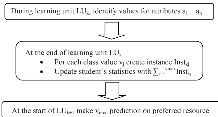
Fig. 2. Naïve Bayes classifier algorithm
